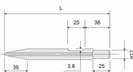
タガネ表 (CHISELS LIST)
